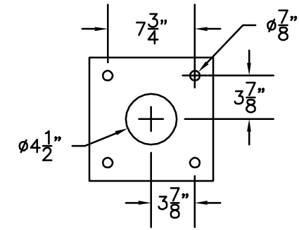
PEDESTAL BOLT PATTERN
